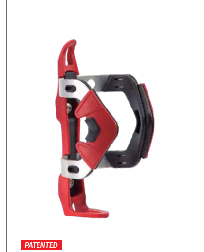
PATENTED YAB-28 Alloy Adjustable 3-position bottle shifting: right, central, left side bottle removal Plastic pads to fit various bottle sizes
