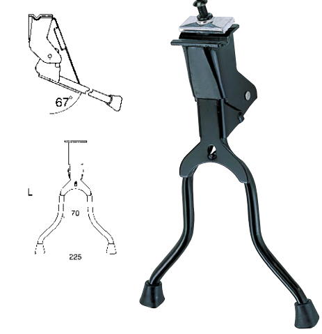
E-bikes/ City / Commuter / Touring YCD-3 Steel mounting seat, steel tube stays
