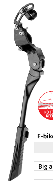
SPECIALLY DESIGNED ANGLE The bracket can be retracted under the chainstays when it is kicked up and will not protrude, preventing your heels from being accidentally hit. E-bikes / City / Commuter / MTB YRA-81BA ADC10 with plastic feet Big angle, fit bikes with disc brakes Adjustable: 24" - 29" Max. weight: 25 kg
